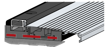
Cutouts properly locate fasteners on substrate Render depicts Z-FEN Sill with red highlights showing cutouts.
